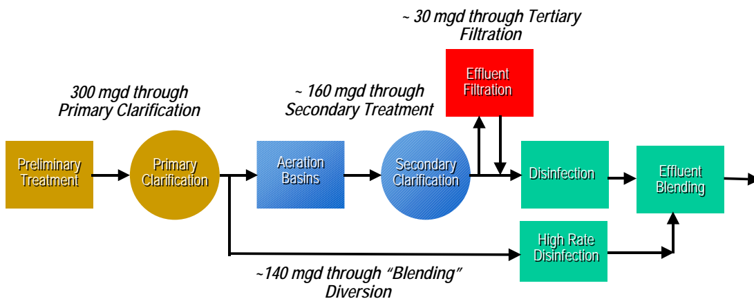
FIGURE 2 Process Flow Schematic for Alternative 1—Additional Primary Clarifiers MWMC Facility Plan, Eugene-Springfield
