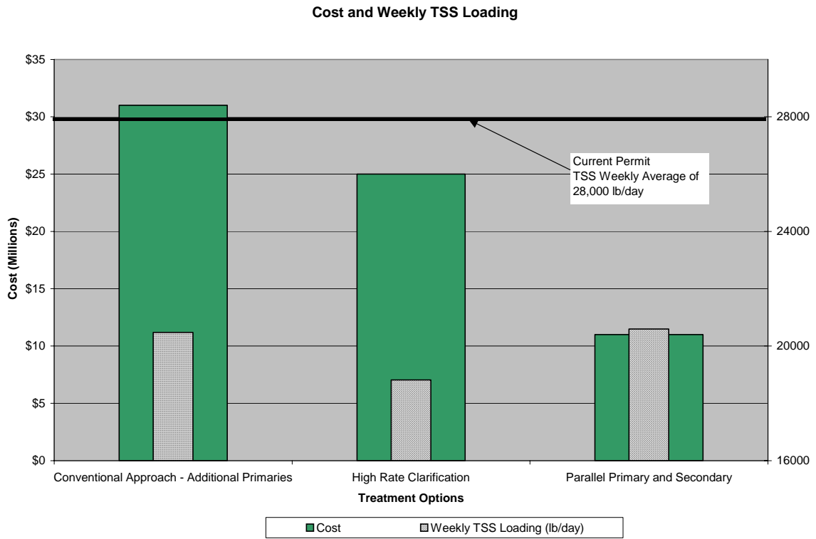
FIGURE 8 Cost and Weekly TSS Loading MWMC Facility Plan, Eugene-Springfield
