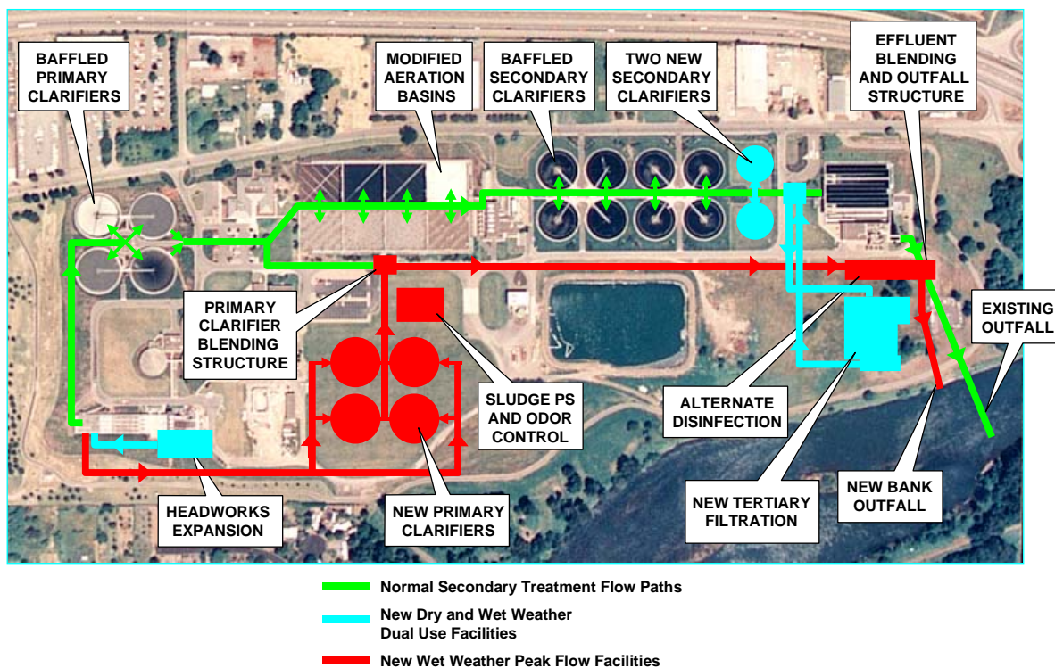
FIGURE 3 Proposed Layout for Alternative 1—Additional Primary Clarifiers MWMC Facility Plan, Eugene-Springfield
