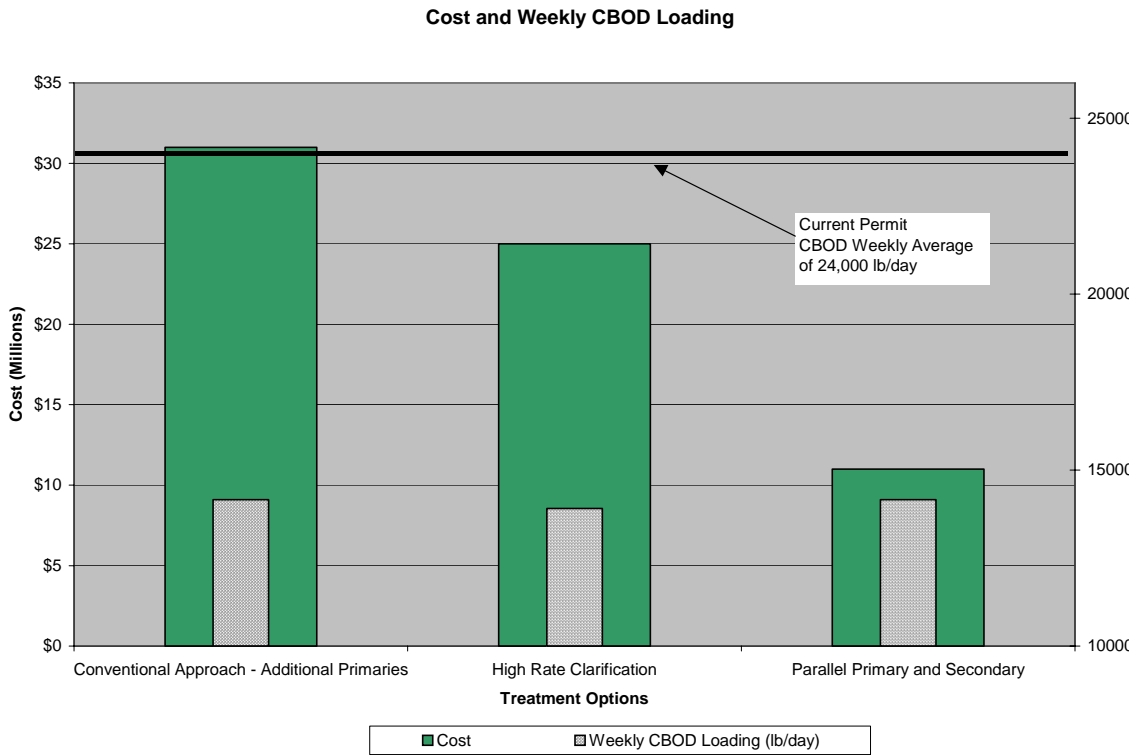
FIGURE 9 Cost and Weekly CBOD 5 Loading MWMC Facility Plan, Eugene-Springfield
