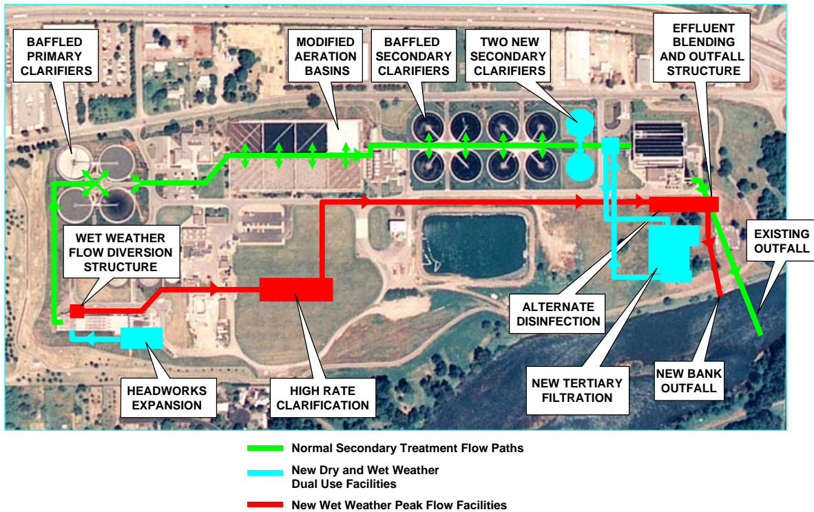
FIGURE 5 Proposed Layout Alternative 2—HRC MWMC Facility Plan, Eugene-Springfield
