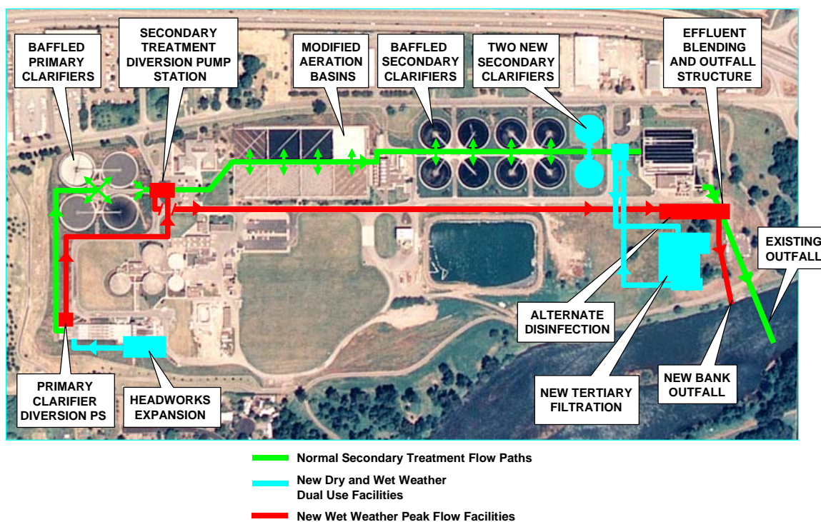
FIGURE 7 Proposed Layout Alternative 3—Parallel Primary and Secondary Treatment MWMC Facility Plan, Eugene-Springfield
