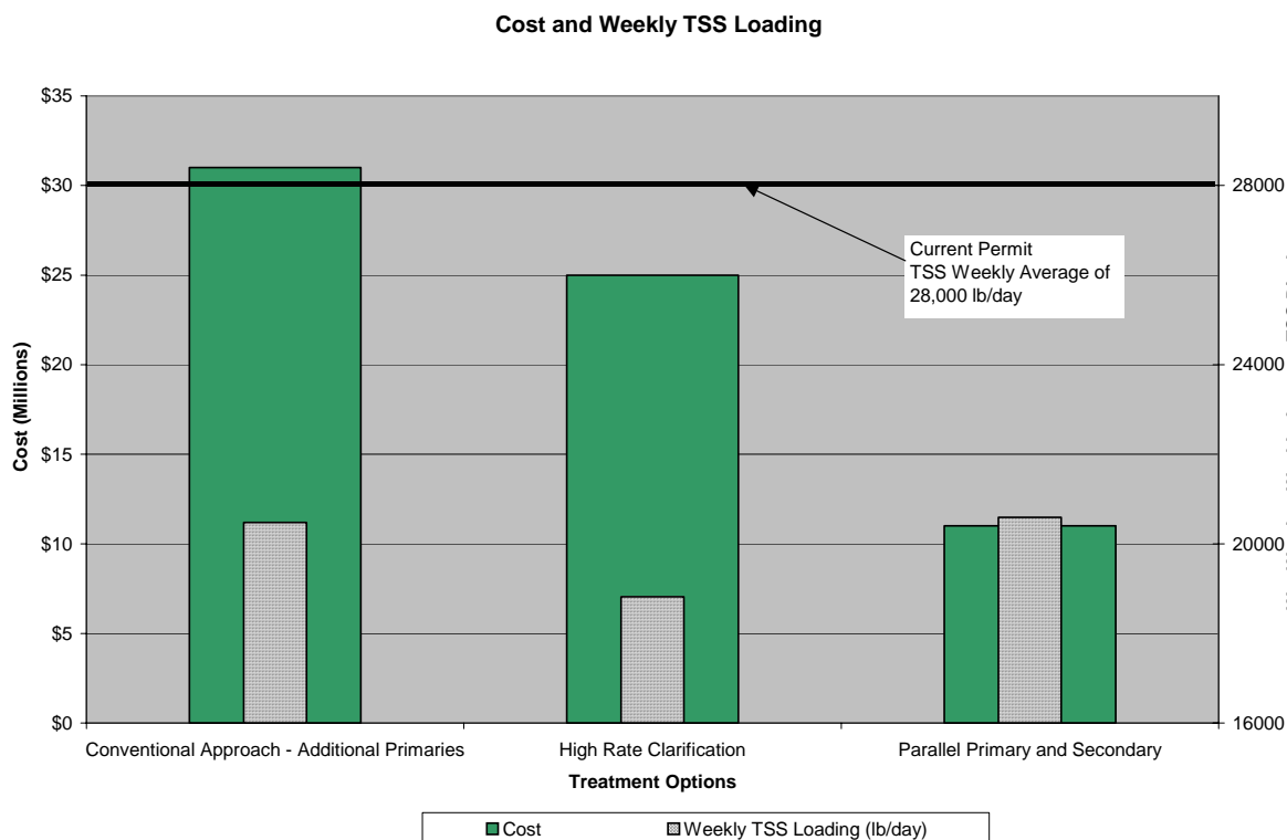
FIGURE 1 Anticipated Weekly TSS Loadings and Relative Costs MWMC Facility Plan, Eugene-Springfield
