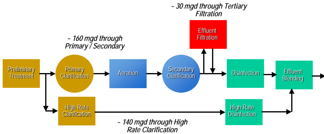
FIGURE 4 Process Flow Schematic Alternative 2—HRC MWMC Facility Plan, Eugene-Springfield
