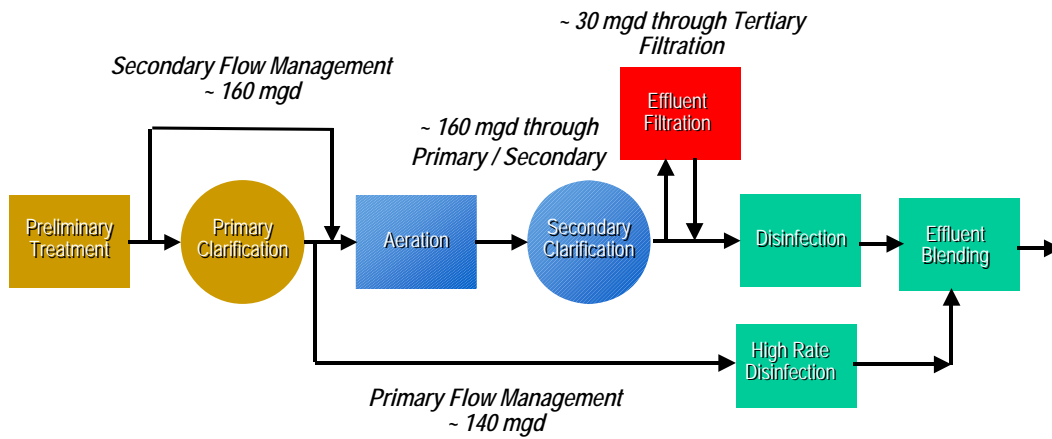
FIGURE 6 Process Flow Diagram Alternative 3—Parallel Primary and Secondary MWMC Facility Plan, Eugene-Springfield
